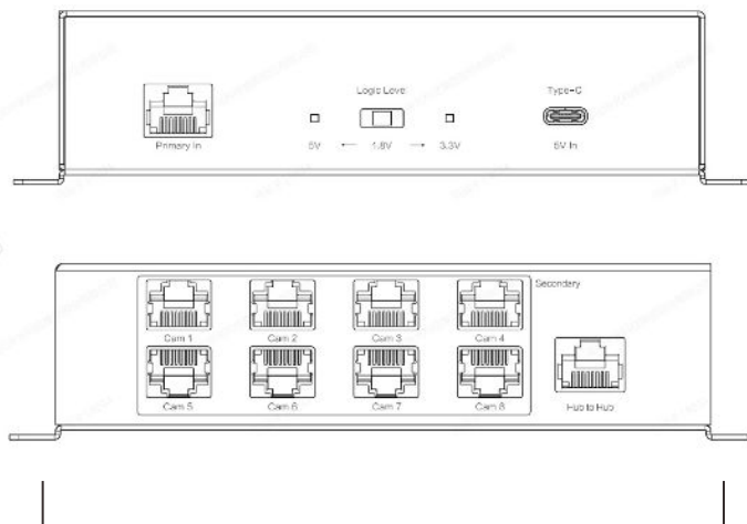
Front and Rear view of the Multi-Camera Sync Hub Pro
